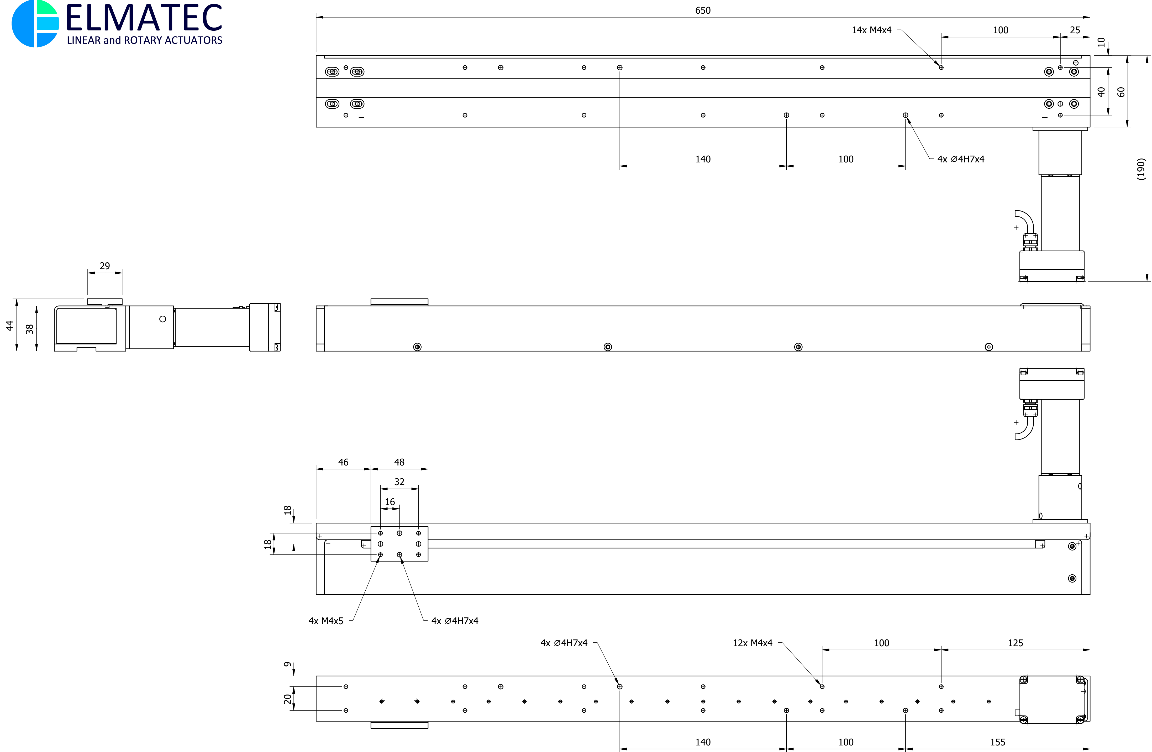
LA-BDTP-130 with stroke 500 (510 mm) with drive FAULHABER 3268BX4-Cx
